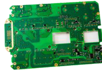
On-board charger electronics VT Automotive Electronics
